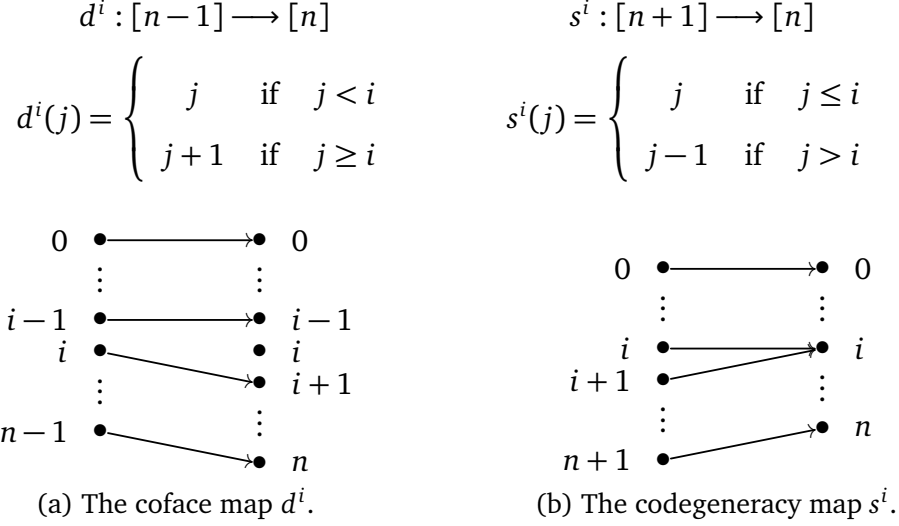
Figure 7.1.1.2: Generators for \Delta
