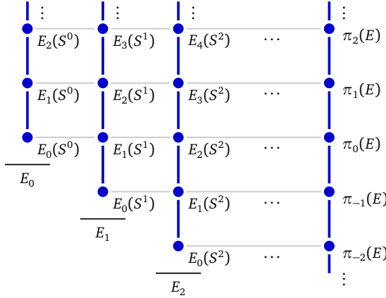
Figure 2.5.2.8: An \Omega -spectrum representing a homology theory. All homology groups are reduced.
