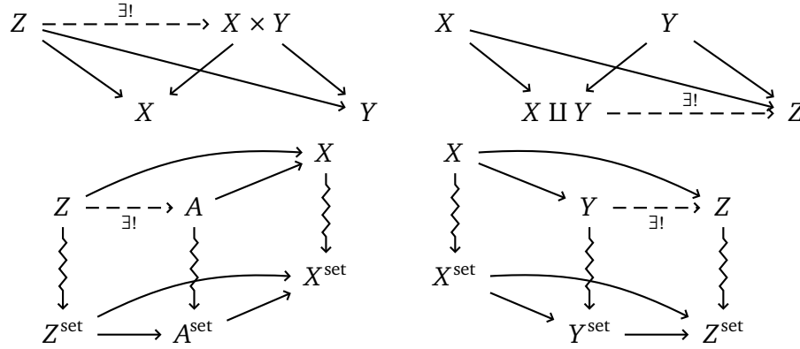
Figure 1.1.1.1: The defining properties of products, coproducts, subspaces, and quotients.
