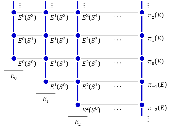
Figure 2.5.2.9: The same \Omega -spectrum representing a cohomology theory. All cohomology groups are reduced.
